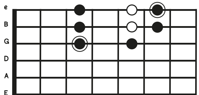
Lydian Dominant = 1 2 3 #4 5 6 b7
