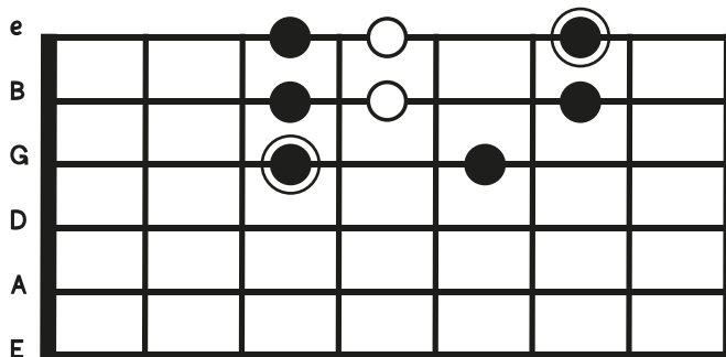
Ionian (aka major scale) = 1 2 3 4 5 6 7
