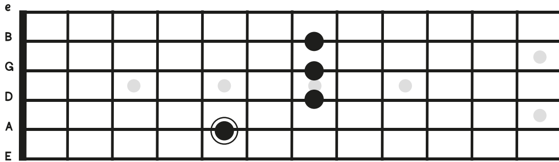
Major Chord with Root on the A String
